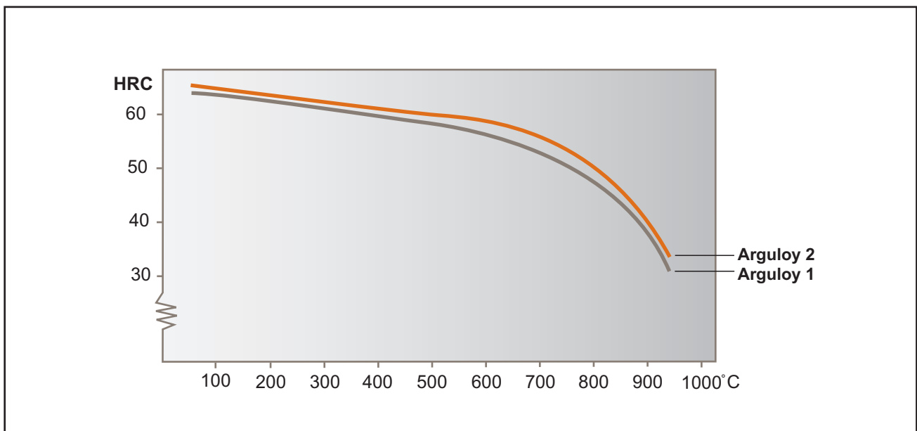
Bild 8 Warmhärte verschiedener Arguloy-Typen Figure 8 Elevated temperature hardness of various Arguloy types
